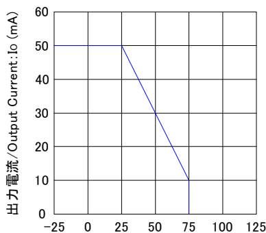
Output Current vs. Ambient Temperature
